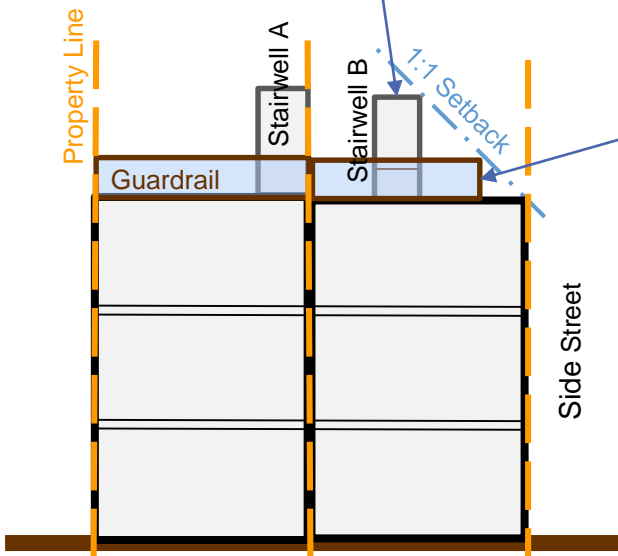
Elevation View from the Front Street
