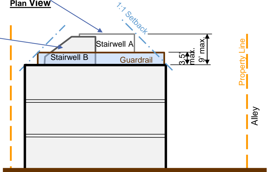
Elevation View from the Side Street
